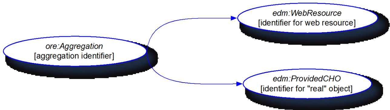
Figure 1. The three core classes: an Aggregation with a Provided CHO and a Web Resource
