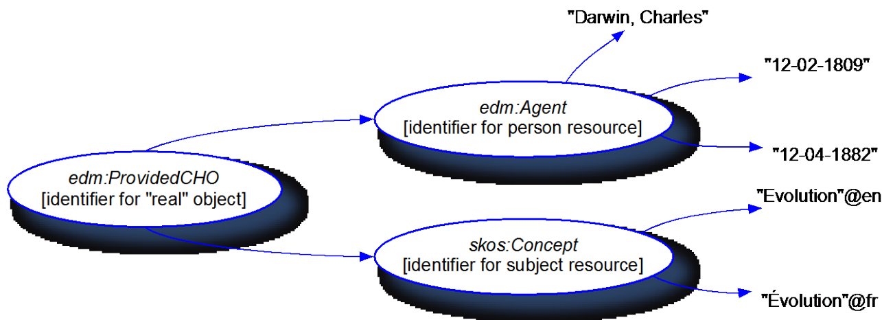
Figure 2. A Provided CHO with two contextual resources
